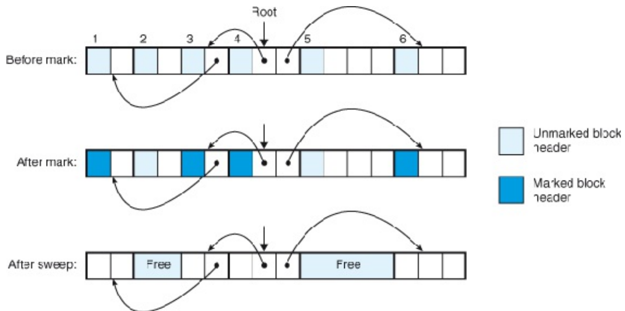
Figure 9.52 Mark&Sweep example.
