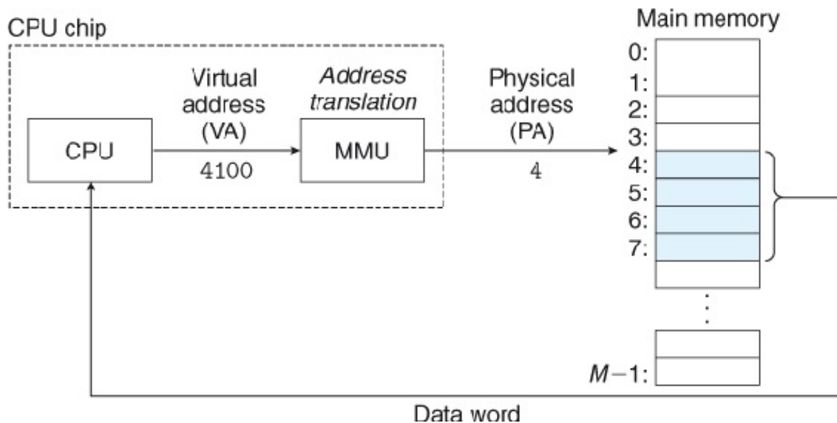
Figure 9.2 A system that uses virtual addressing.
