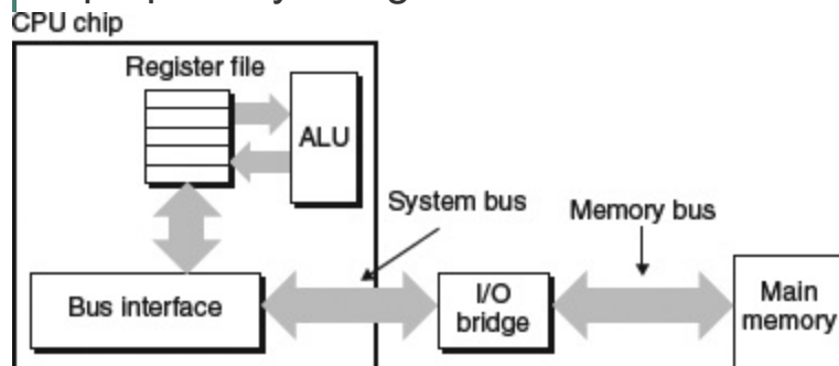
Figure 6.6 Example bus structure that connects the CPU and main memory.
