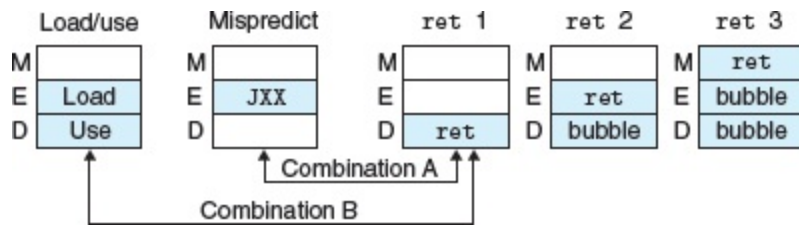
Figure 4.67 Pipeline states for special control conditions.
